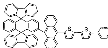
Chemical Compound 133
