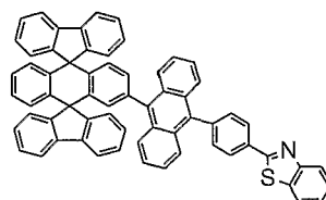
Chemical Compound 217
