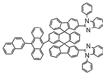
Chemical Compound 222
