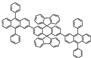
Chemical Compound 122
