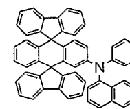
Chemical Compound 301
