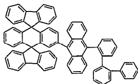
Chemical Compound 112
