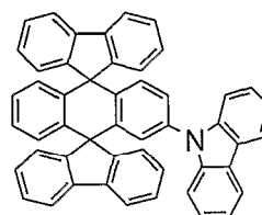
Chemical Compound 10
