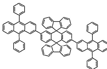
Chemical Compound 122
