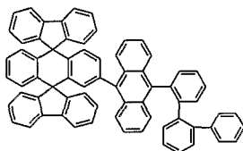
Chemical Compound 112
