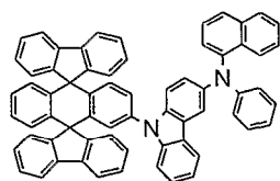
Chemical Compound 306
