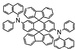
Chemical Compound 302
