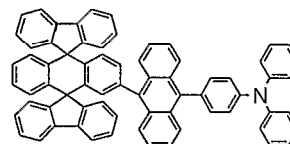
Chemical Compound 401
