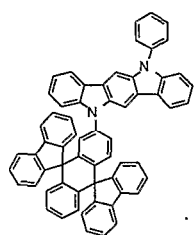
Chemical Compound 408
