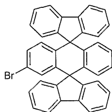
15 Chemical Compound 1
