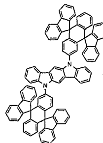
Chemical Compound 405
