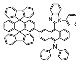
Chemical Compound 127
