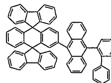
Chemical Compound 111
