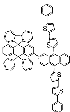
Chemical Compound 128
