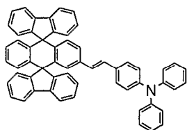
Chemical Compound 400
