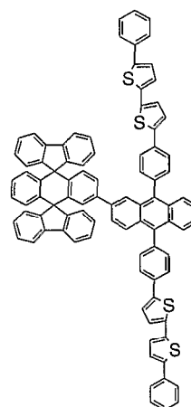
Chemical Compound 129
