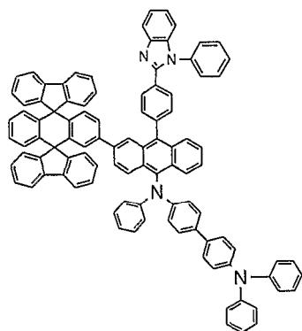
Chemical Compound 124
