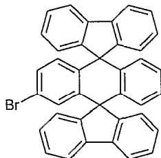
Chemical Compound 1
