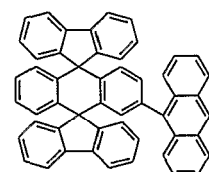
Chemical Compound 9
