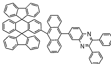
Chemical Compound 203
