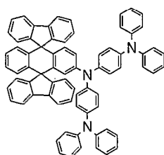
Chemical Compound 308
