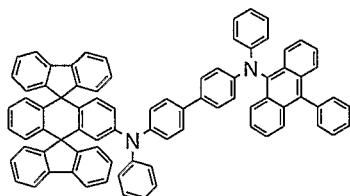
Chemical Compound 408
