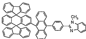
Chemical Compound 208
