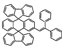
Chemical Compound 106
