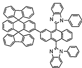
Chemical Compound 202
