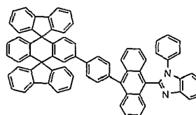
Chemical Compound 207
