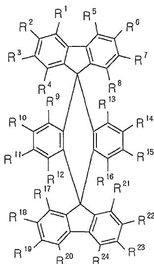
General Formula 1
