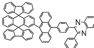
Chemical Compound 209
