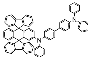
Chemical Compound 307
