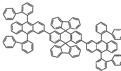
Chemical Compound 121
