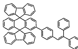
Chemical Compound 107
