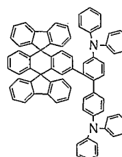
Chemical Compound 305
