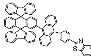
Chemical Compound 217
