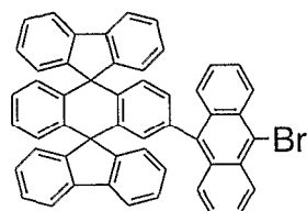
Chemical Compound 5
