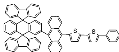
Chemical Compound 132
