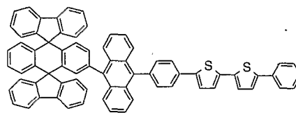
Chemical Compound 131
