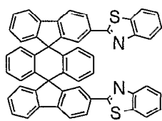
Chemical Compound 220
