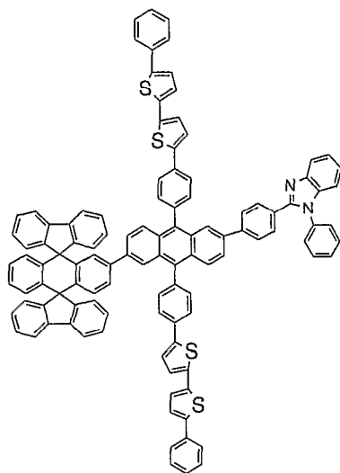
Chemical Compound 130
