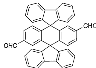
Chemical Compound 4
