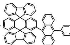
Chemical Compound 109
