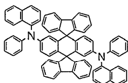
Chemical Compound 302
