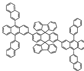
Chemical Compound 123
