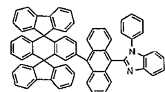
Chemical Compound 200
