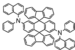
Chemical Compound 302
