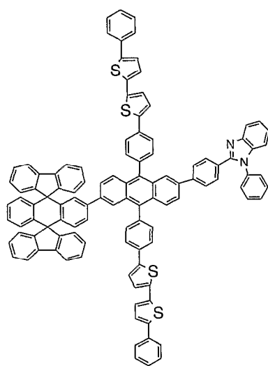
Chemical Compound 130
