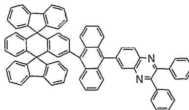
Chemical Compound 203
