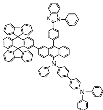
Chemical Compound 124
