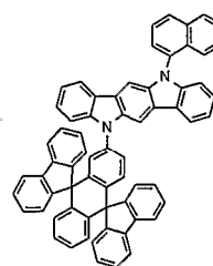
Chemical Compound 409
