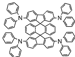
Chemical Compound 304
