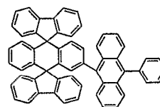
Chemical Compound 109
