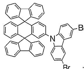
Chemical Compound 6
