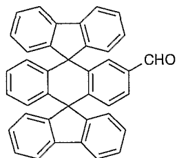
Chemical Compound 3
