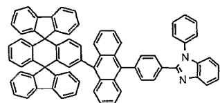
Chemical Compound 204
