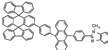
Chemical Compound 211
