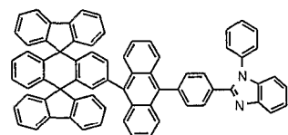
Chemical Compound 204
