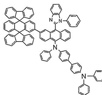
Chemical Compound 125
