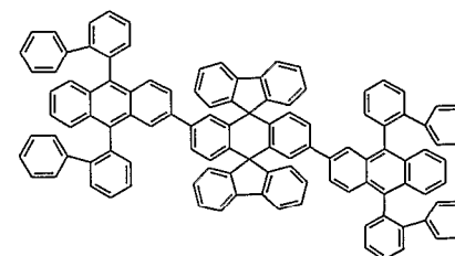
Chemical Compound 121
