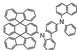
Chemical Compound 306
