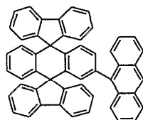
Chemical Compound 9
