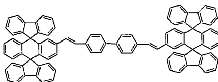
Chemical Compound 100
