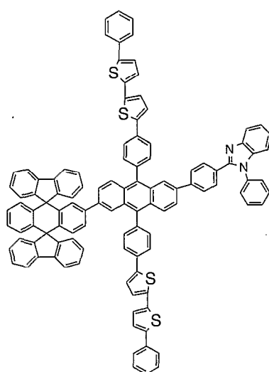
Chemical Compound 130
