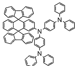
Chemical Compound 308
