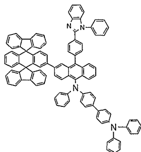
Chemical Compound 124
