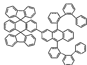
Chemical Compound 136
