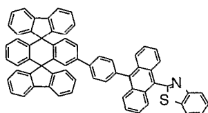
Chemical Compound 216
