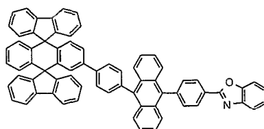
Chemical Compound 126
