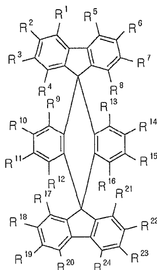
Chemical Formula 1
