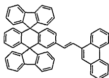
Chemical Compound 104
