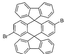
Chemical Compound 2
