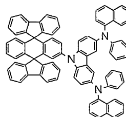
Chemical Compound 403
