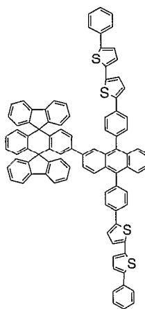
Chemical Compound 129
