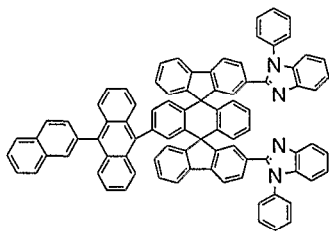
Chemical Compound 222
