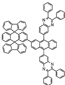
Chemical Compound 212
