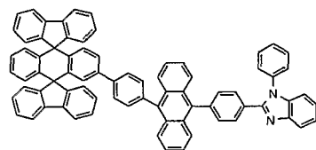
Chemical Compound 210
