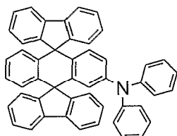
Chemical Compound 11
