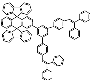
Chemical Compound 108
