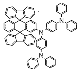
Chemical Compound 308
