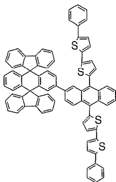
Chemical Compound 128
