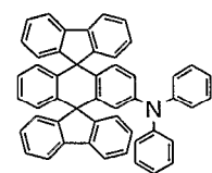
Chemical Compound 300
