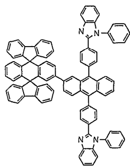
Chemical Compound 206
