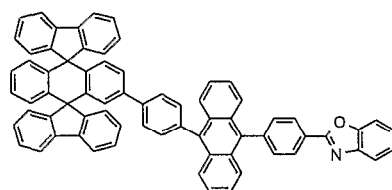
Chemical Compound 126
