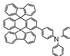
Chemical Compound 303
