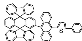
Chemical Compound 134
