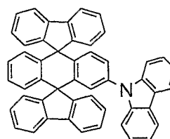
Chemical Compound 10
