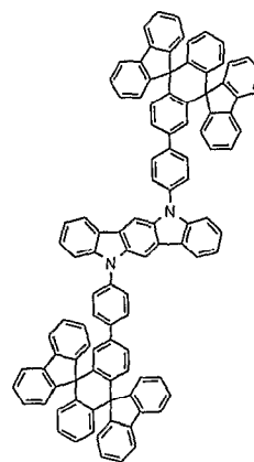
Chemical Compound 409
