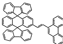
Chemical Compound 104
