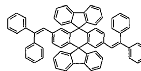
Chemical Compound 105
