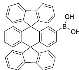
Chemical Compound 8
