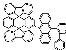
Chemical Compound 111
