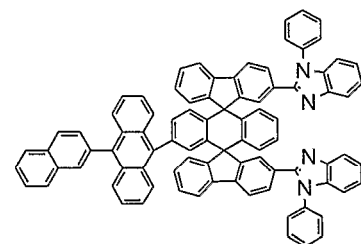
Chemical Compound 222
