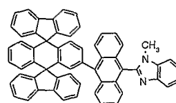
Chemical Compound 205
