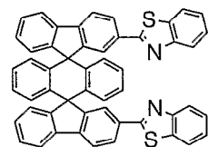
Chemical Compound 220
