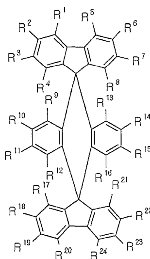
Chemical Formula 1
