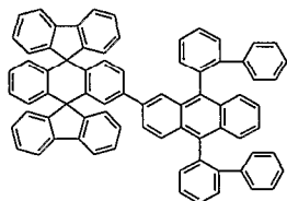
Chemical Compound 118
