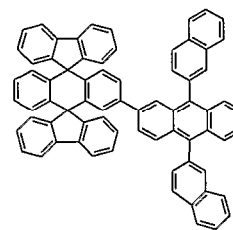
Chemical Compound 117
