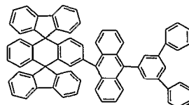
Chemical Compound 113
