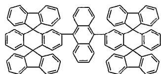
Chemical Compound 102
