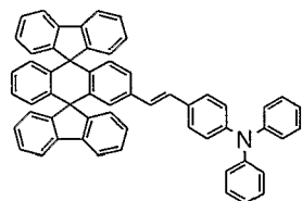
Chemical Compound 400
