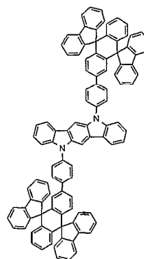
Chemical Compound 409
