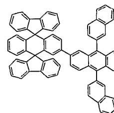
Chemical Compound 117
