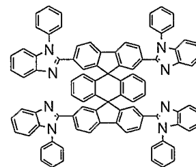
Chemical Compound 219
