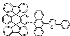
Chemical Compound 134
