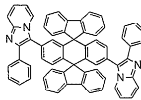
Chemical Compound 413.
