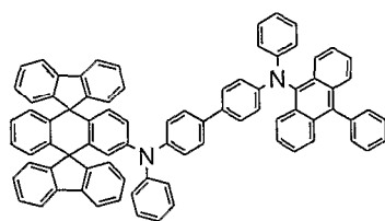
Chemical Compound 408
