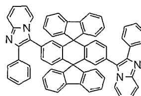
Chemical Compound 413.
