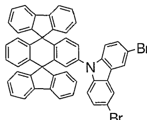
Chemical Compound 6
