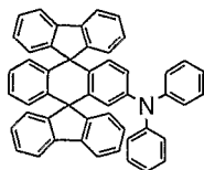
Chemical Compound 300
