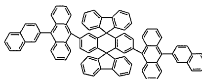
Chemical Compound 115
