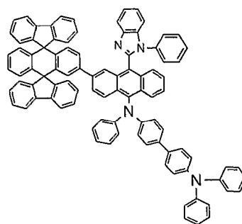
Chemical Compound 125
