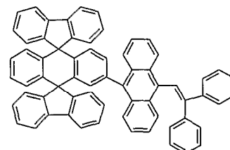
Chemical Compound 137
