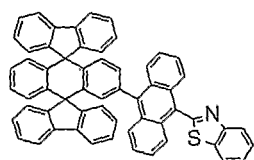
Chemical Compound 214
