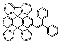
Chemical Compound 106
