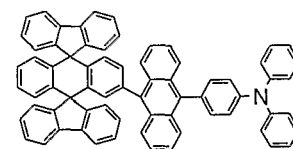
Chemical Compound 401
