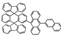
Chemical Compound 110
