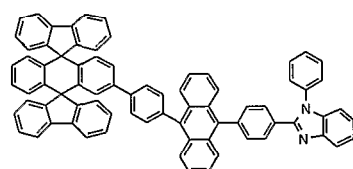
Chemical Compound 210
