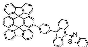
Chemical Compound 216
