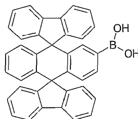
Chemical Compound 8
