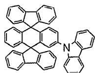
Chemical Compound 404
