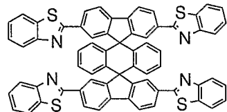
Chemical Compound 218
