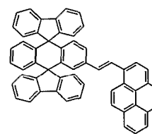
Chemical Compound 103
