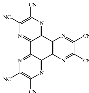
Hexanitrile hexaazatriphenylene
