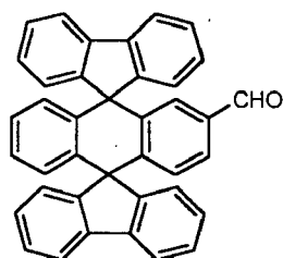
Chemical Compound 3
