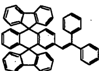
Chemical Compound 106
