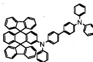
Chemical Compound 307
