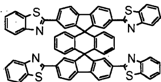
Chemical Compound 218
