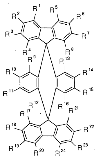
General Formula 1
