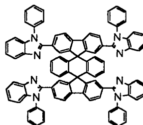
Chemical Compound 219
