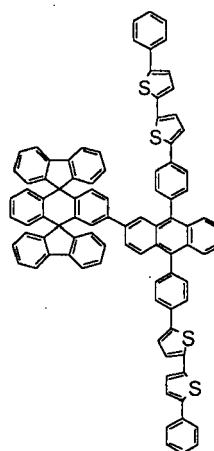
Chemical Compound 129
