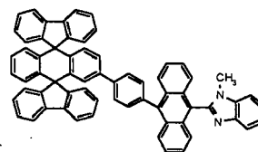
Chemical Compound 201
