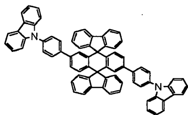
Chemical Compound 402
