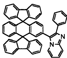
Chemical Compound 412
