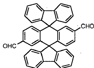
Chemical Compound 4
