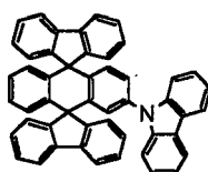
Chemical Compound 404
