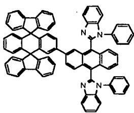
Chemical Compound 202
