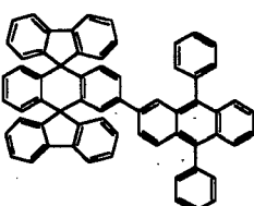
Chemical Compound 116
