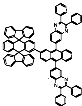
Chemical Compound 212
