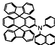
Chemical Compound 301
