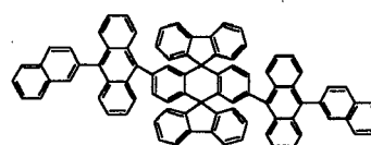
Chemical Compound 115
