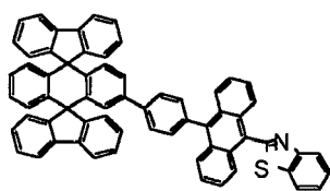
Chemical Compound 216
