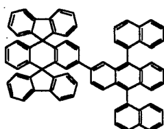
Chemical Compound 120
