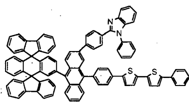
Chemical Compound 132
