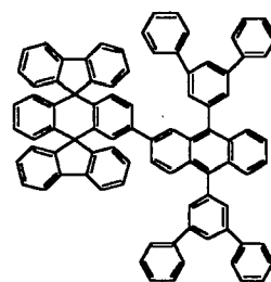
Chemical Compound 119
