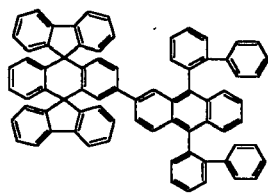
Chemical Compound 118
