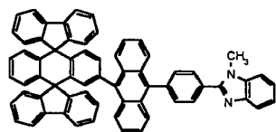
Chemical Compound 208
