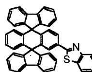
Chemical Compound 215
