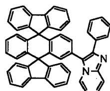
Chemical Compound 412
