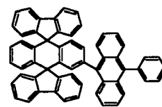
Chemical Compound 109
