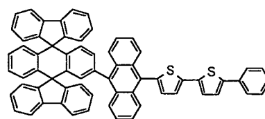
Chemical Compound 133
