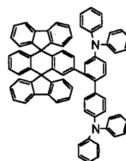
Chemical Compound 305
