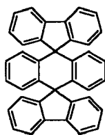
Chemical Compound 12
