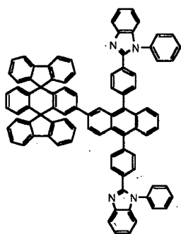
Chemical Compound 206
