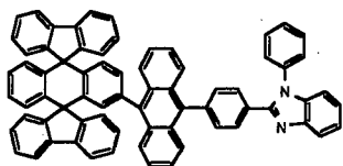
Chemical Compound 204
