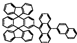
Chemical Compound 110
