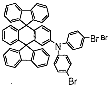
Chemical Compound 7
