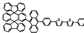
Chemical Compound 131
