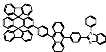
Chemical Compound 210
