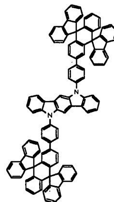
Chemical Compound 409
