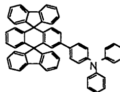
Chemical Compound 303
