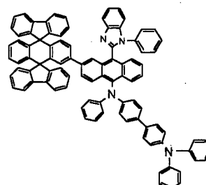
Chemical Compound 125
