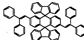
Chemical Compound 105
