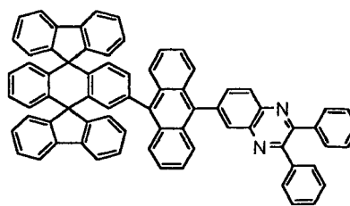
Chemical Compound 203
