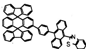
Chemical Compound 216
