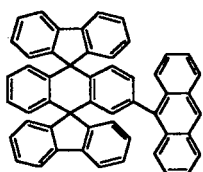
Chemical Compound 9
