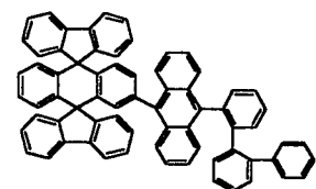
Chemical Compound 112
