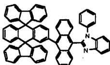
Chemical Compound 200
