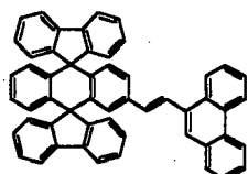
Chemical Compound 104
