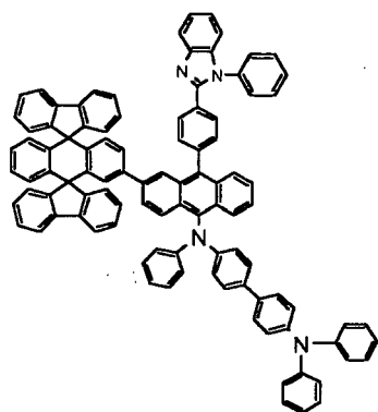
Chemical Compound 124
