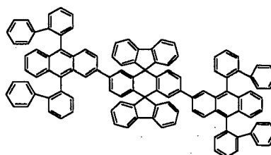
Chemical Compound 121
