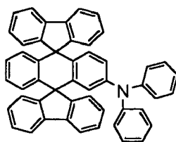
Chemical Compound 11
