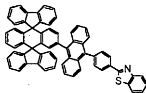
Chemical Compound 217
