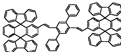
Chemical Compound 101
