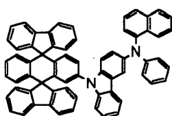
Chemical Compound 306
