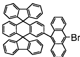
Chemical Compound 5
