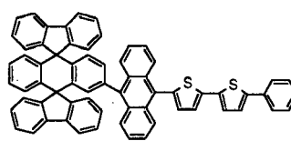
Chemical Compound 133
