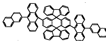
Chemical Compound 115
