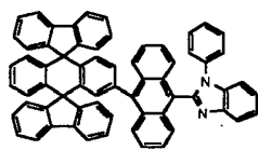
Chemical Compound 200
