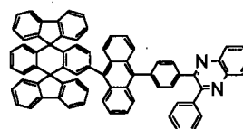
Chemical Compound 209
