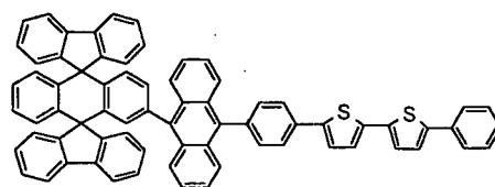
Chemical Compound 131
