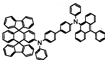
Chemical Compound 408
