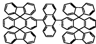
Chemical Compound 102
