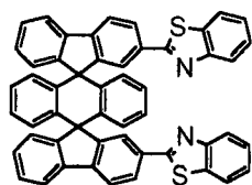
Chemical Compound 220
