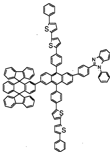
Chemical Compound 130
