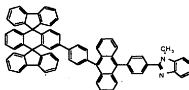
Chemical Compound 211
