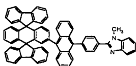
Chemical Compound 208
