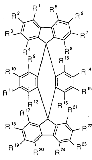
Chemical Formula 1
