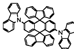
Chemical Compound 407
