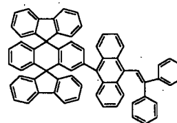
Chemical Compound 137
