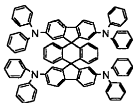
Chemical Compound 304
