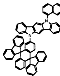
Chemical Compound 411
