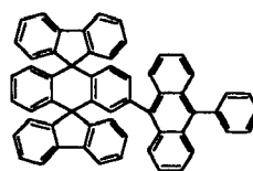
Chemical Compound 109
