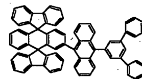
Chemical Compound 113
