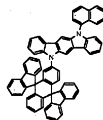
Chemical Compound 411
