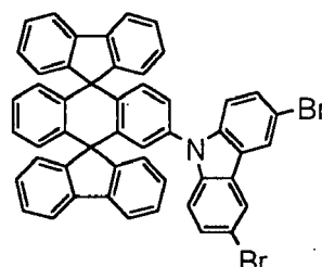
Chemical Compound 6
