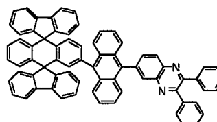
Chemical Compound 203
