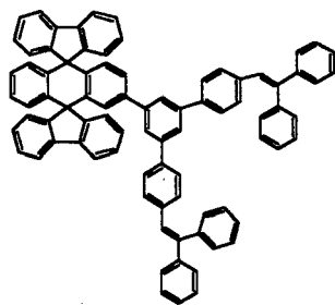
Chemical Compound 108
