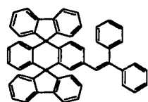
Chemical Compound 106
