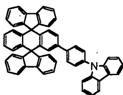
Chemical Compound 406
