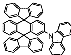
Chemical Compound 10
