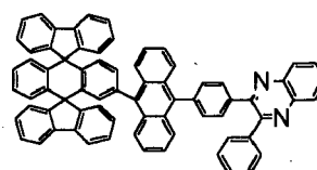
Chemical Compound 209
