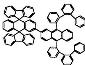
Chemical Compound 136
