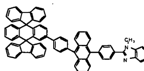
Chemical Compound 211
