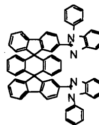
Chemical Compound 221
