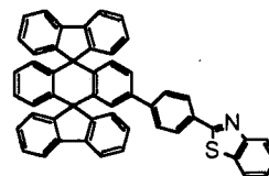
Chemical Compound 213
