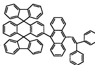
Chemical Compound 137
