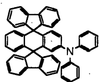
Chemical Compound 300
