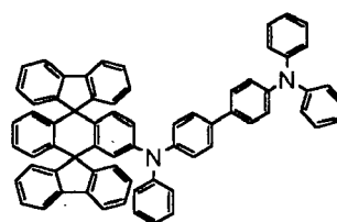
Chemical Compound 307
