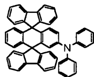
Chemical Compound 300
