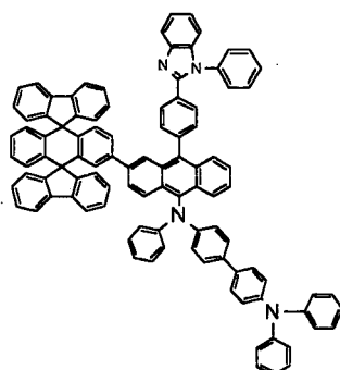
Chemical Compound 124
