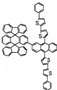
Chemical Compound 128
