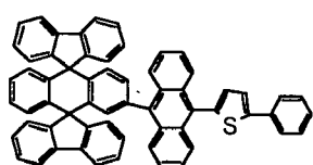
Chemical Compound 134
