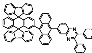
Chemical Compound 203
