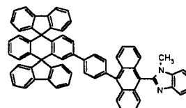
Chemical Compound 201
