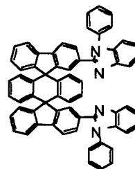
Chemical Compound 221
