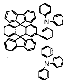
Chemical Compound 305
