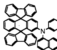
Chemical Compound 301
