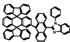
Chemical Compound 200
