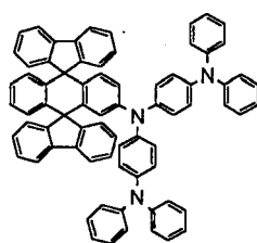
Chemical Compound 308
