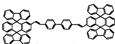
Chemical Compound 100
