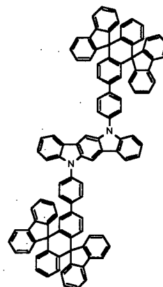
Chemical Compound 409
