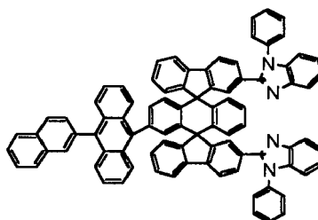
Chemical Compound 222.
