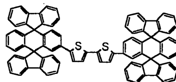
Chemical Compound 135
