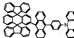
Chemical Compound 401
