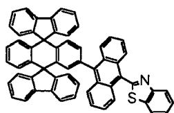
Chemical Compound 214
