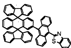
Chemical Compound 214
