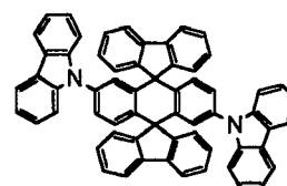
Chemical Compound 407
