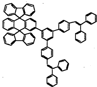
Chemical Compound 108
