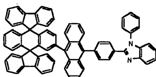
Chemical Compound 204
