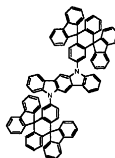
Chemical Compound 405
