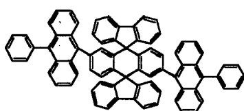
Chemical Compound 114
