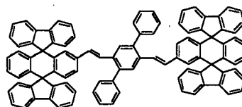
Chemical Compound 101
