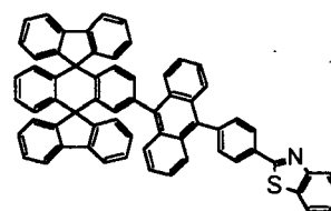
Chemical Compound 217
