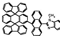
Chemical Compound 205
