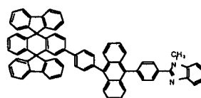
Chemical Compound 211
