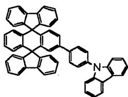
Chemical Compound 406
