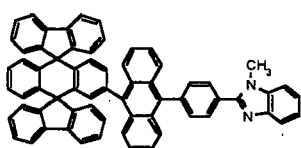
Chemical Compound 208
